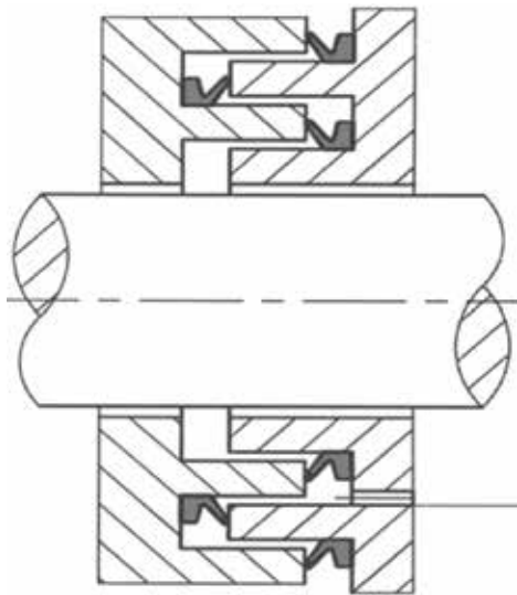
TENUTE A LABIRINTO | LABYRINTH SYSTEM
